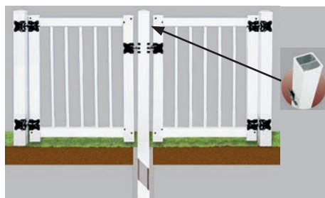
Removable Center Post is Recommended on Double Gates.
