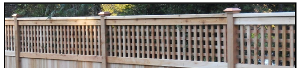
Square Lattice
